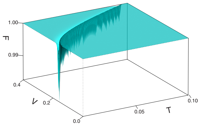
FIG. 7. (Color online) Fidelity F = F(T, V) as a function of the temperature T and the coupling constant V . The plot is given in rescaled quantities T \rightarrow k_B T / (\hbar \omega_D) and V \rightarrow D_F V , with \delta T = 0 and \delta V = 10^{-3} .
