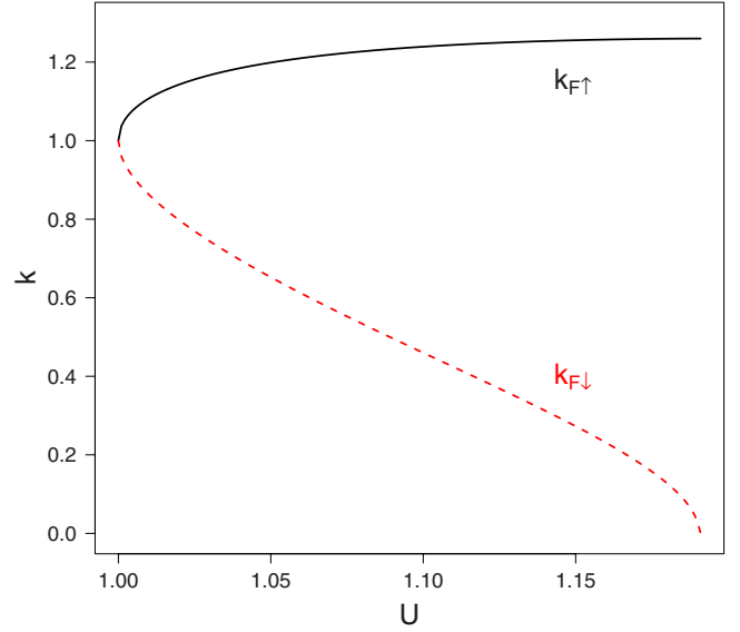
FIG. 1. (Color online) Explicit dependencies k_{F\uparrow} = k_{F\uparrow}(U) (solid line) and k_{F\downarrow} = k_{F\downarrow}(U) (dashed line) determining the ground state (6). Note that at the point of QPT, given by U_c = 1 , the two derivatives dk_{F\uparrow}/dU and dk_{F\downarrow}/dU become infinite, marking the nonanalyticity in the ground state fidelity. The plot is given in rescaled quantities U \rightarrow D_F U and k_{F\sigma} \rightarrow k_{F\sigma}/k_F .
