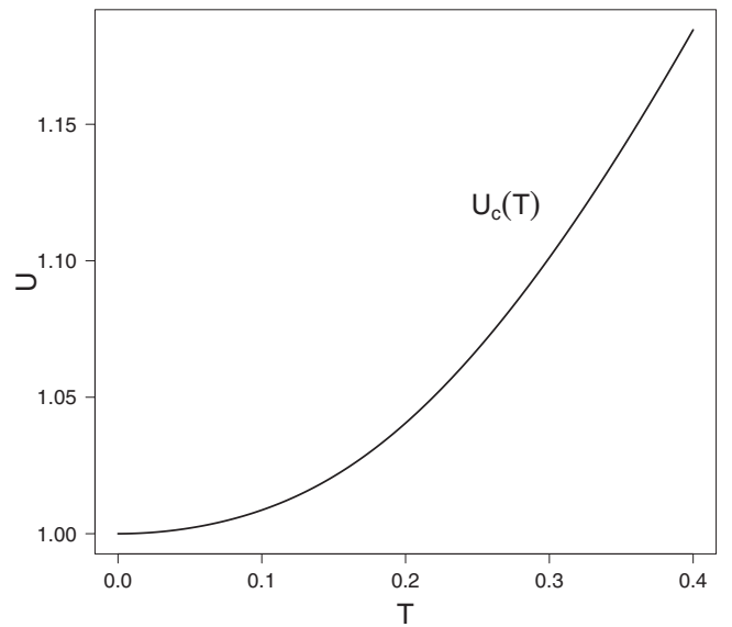
FIG. 3. Critical line of the magnetic phase transition U_c = U_c(T) . The plot is given in rescaled quantities T \rightarrow k_B T and U \rightarrow D_F U .
