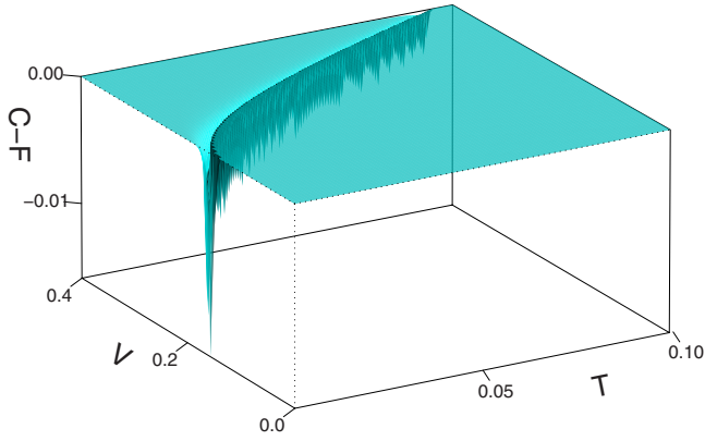
FIG. 8. (Color online) Difference C(T, V) - F(T, V) as a function of the temperature T and the coupling constant V . The plot is given in rescaled quantities T \rightarrow k_B T / (\hbar \omega_D) and V \rightarrow D_F V , with \delta T = 0 and \delta V = 10^{-3} .
