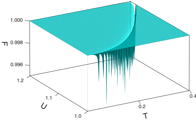
FIG. 4. (Color online) Fidelity F=F(T, U) . The plot is given in rescaled quantities T \rightarrow k_B T and U \rightarrow D_F U , with \delta T=0 and \delta U=2 \times 10^{-3} .
