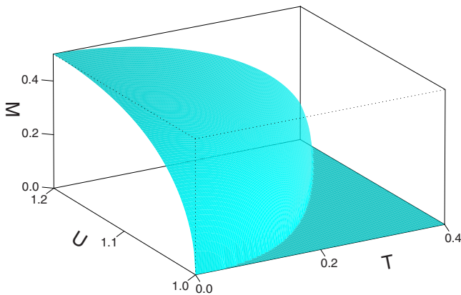
FIG. 2. (Color online) Magnetization M = M(T, U) as a function of the temperature T and the coupling constant U . The plot is given in rescaled quantities T \rightarrow k_B T , U \rightarrow D_F U , and M \rightarrow M/N .
