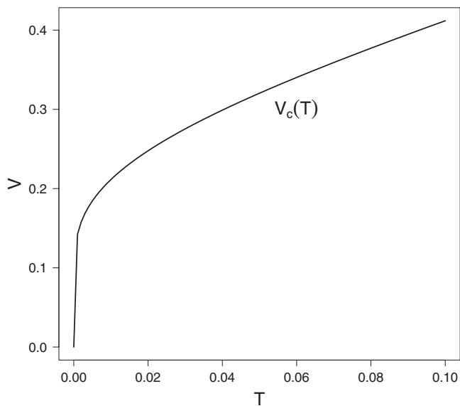
FIG. 6. Critical line V_c = V_c(T) as a function of the temperature T . The plot is given in rescaled quantities T \rightarrow k_B T / (\hbar \omega_D) and V \rightarrow D_F V .
