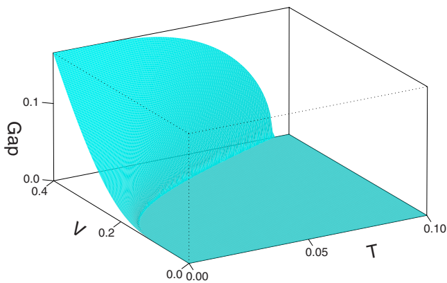
FIG. 5. (Color online) Gap \Delta = \Delta(T, V) as a function of the temperature T and the coupling constant V . The plot is given in rescaled quantities T \rightarrow k_B T / (\hbar \omega_D) , V \rightarrow D_F V , and \Delta \rightarrow \Delta / (\hbar \omega_D) .
